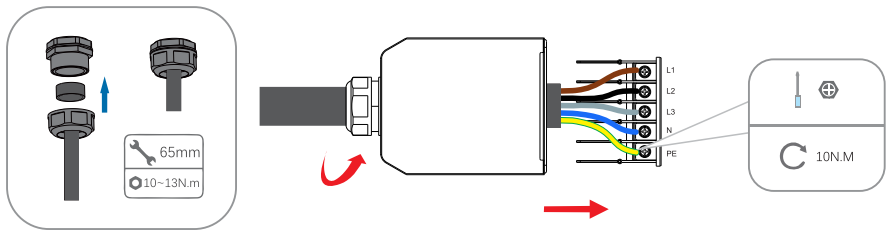
50K AC terminal wiring diagram
